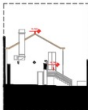
Section 2 1:50
