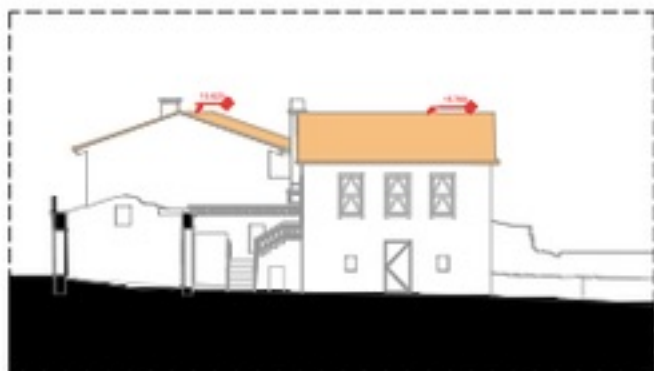
Section 1 1:50
