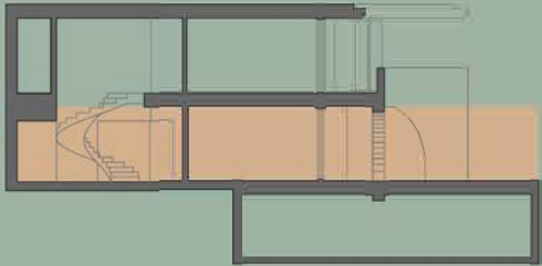
Cortes | Section
