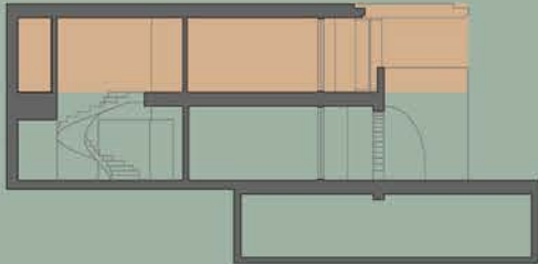
Cortes | Section
