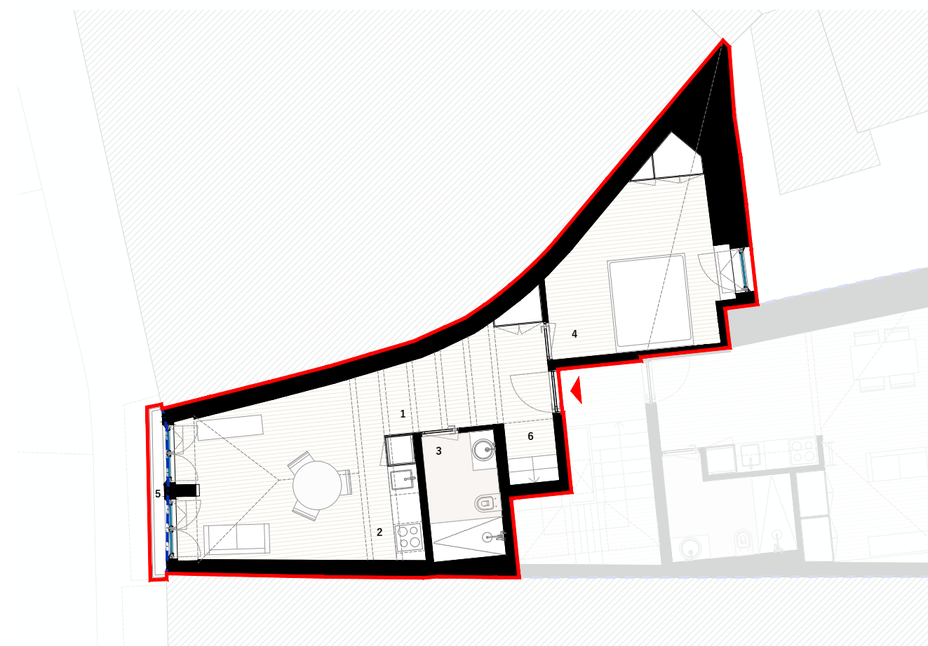
planta piso 3 | 3rd floor plan
