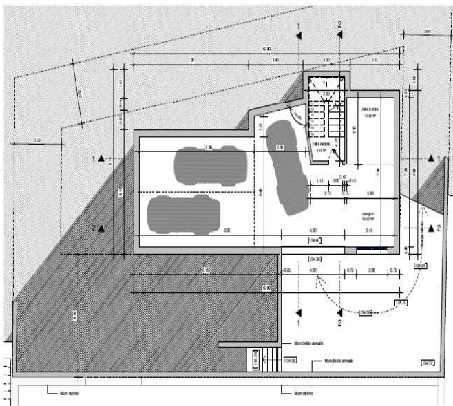
Piano Cave
