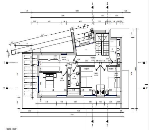
Piano 1
